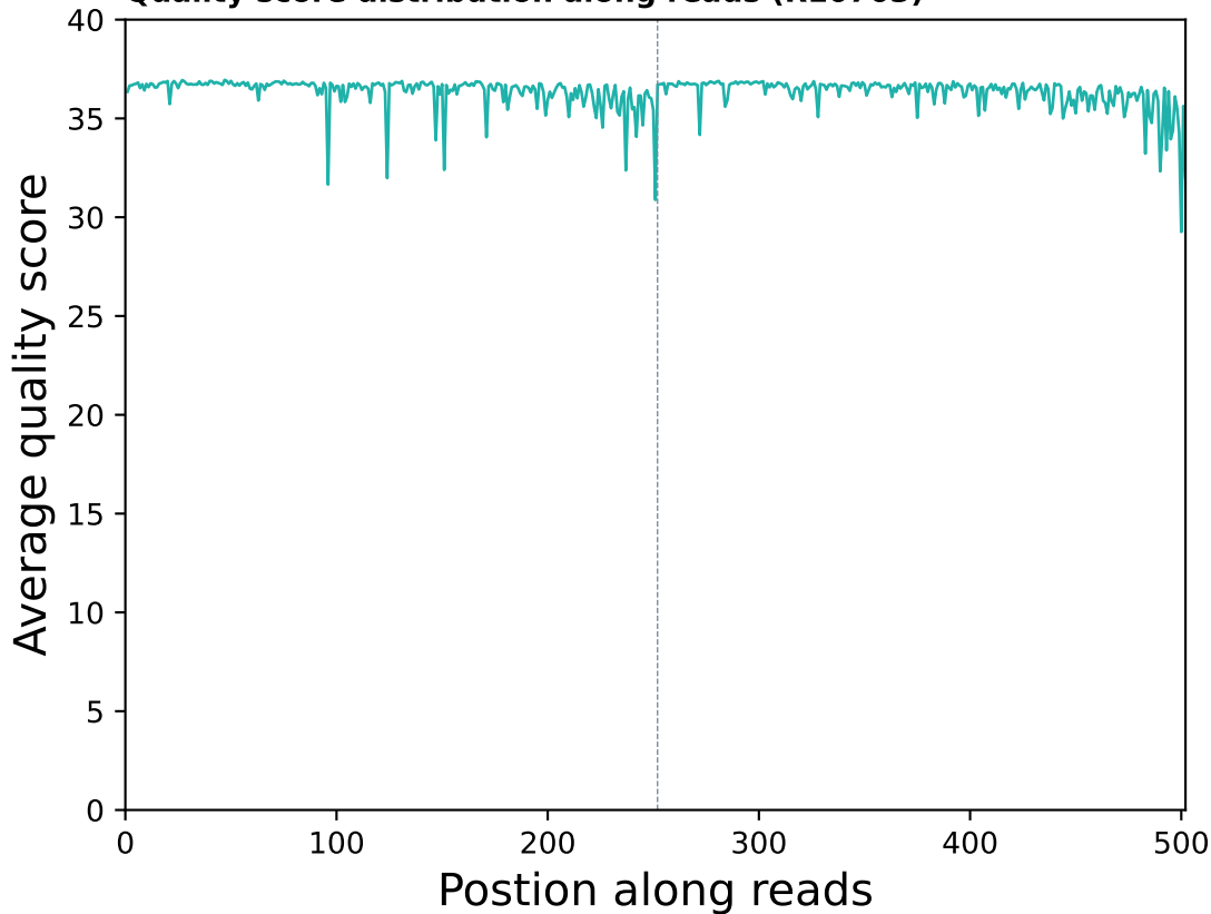
Quality score distribution along reads (R10703)
